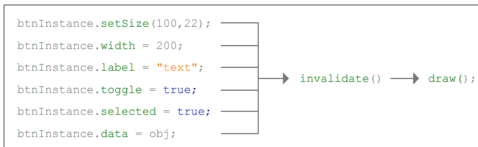
Figure 61: CLIK components automatically invalidate when certain properties are changed.
