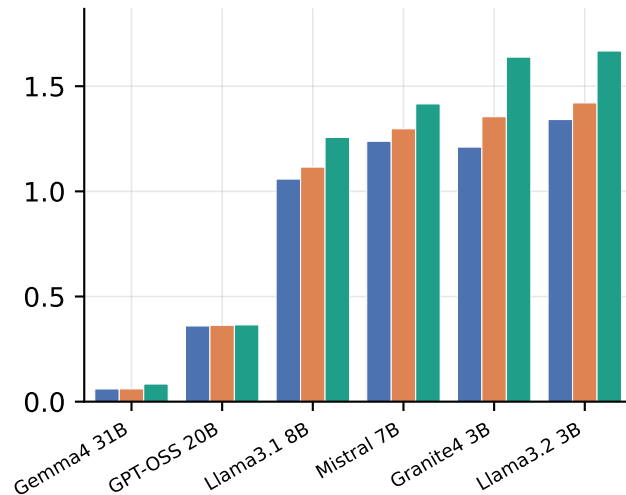
Throughput (cmd/s)
