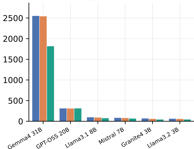
Energy/command (J)
