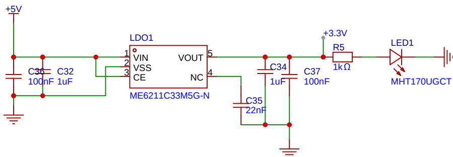
ME6211C33M5G-N LDO电源5V转3.3V
