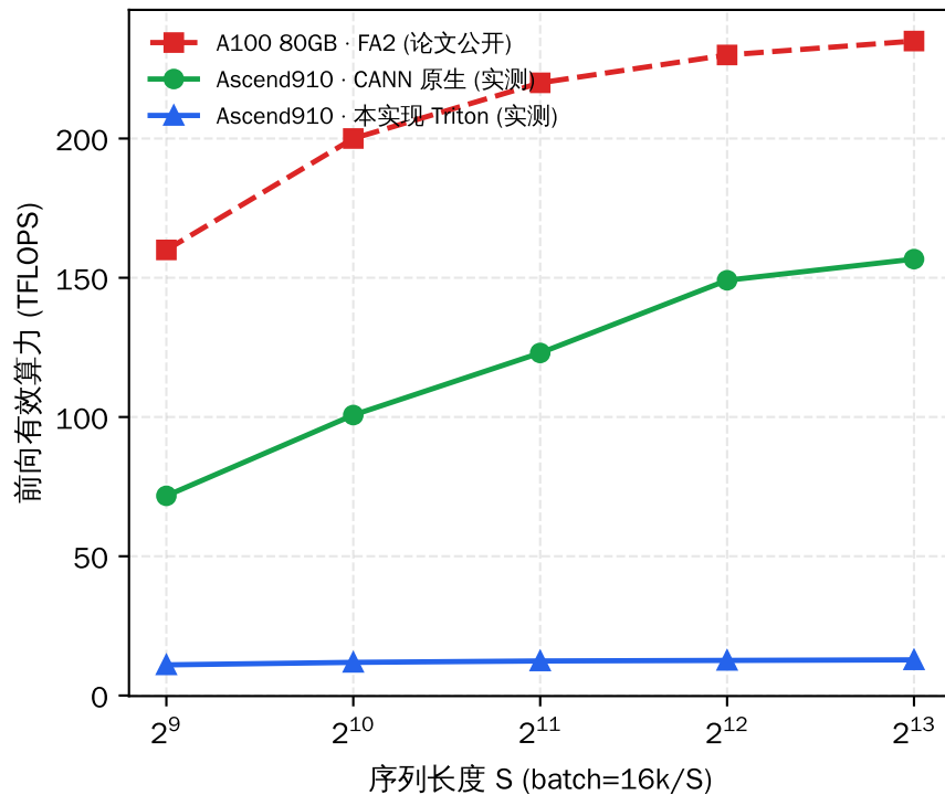
FA2 论文协议对标: Ascend910 vs A100 (fp16, causal, 前向)
