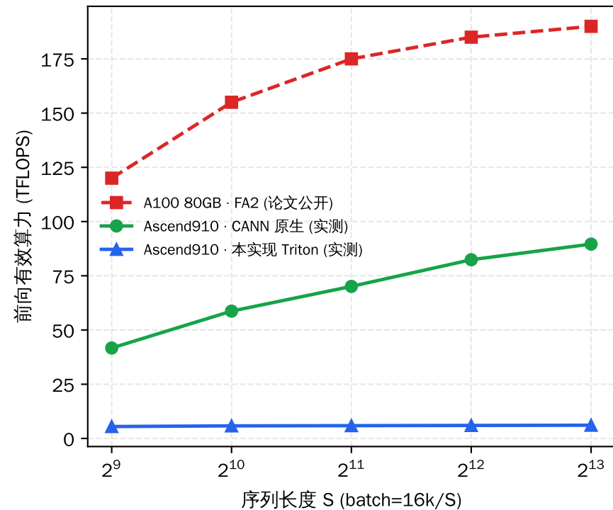
FA2 论文协议对标: Ascend910 vs A100 (fp16, causal, 前向)
