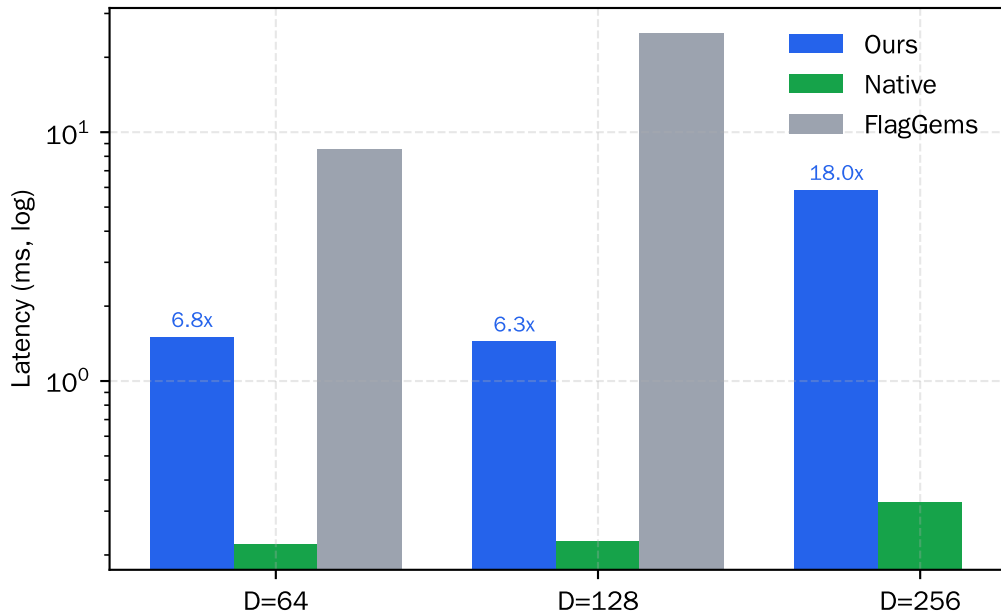
head_dim 扫描 (S=2048, fp16, causal)
