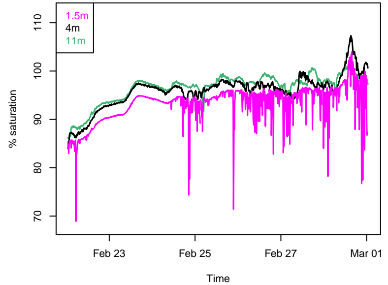
DO % saturation
