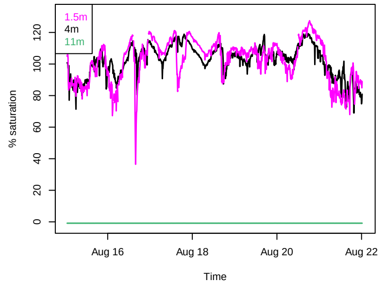
DO % saturation
