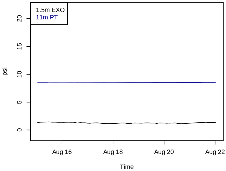
Sonde Pressure
