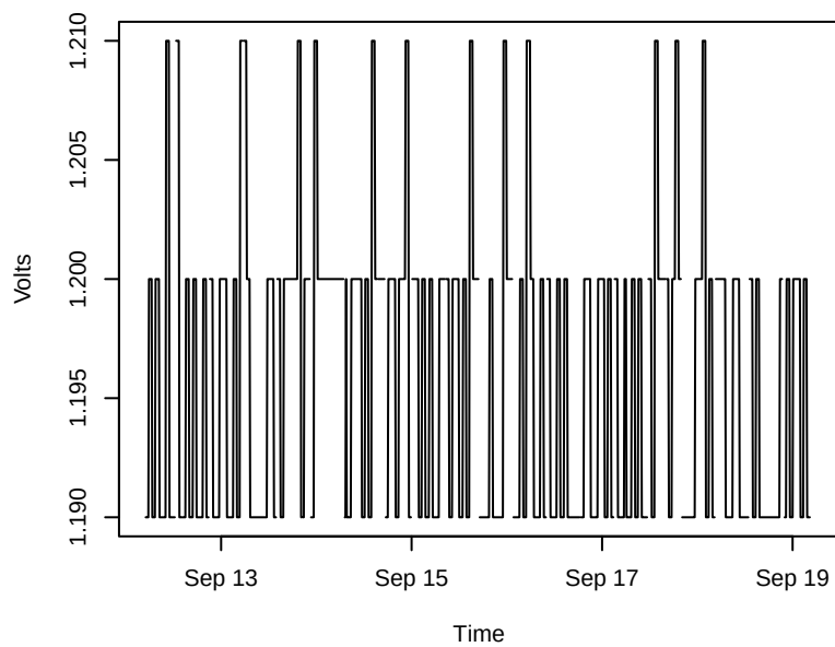
Wiper Voltage
