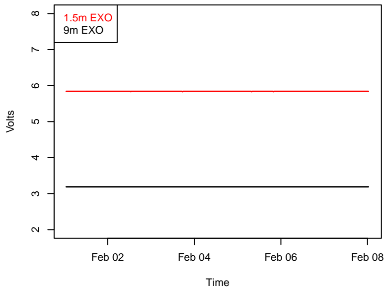
EXO Battery
