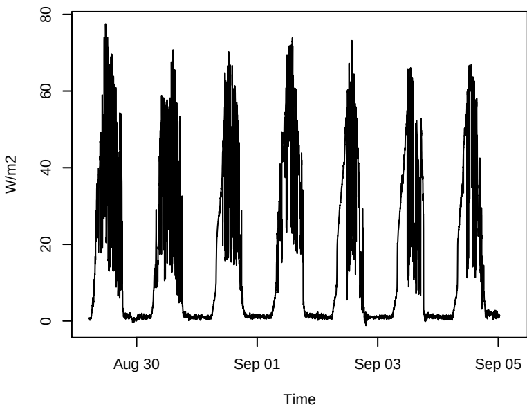
Shortwave Down
