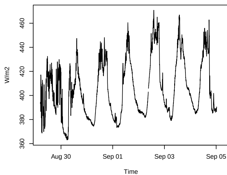
Longwave Up
