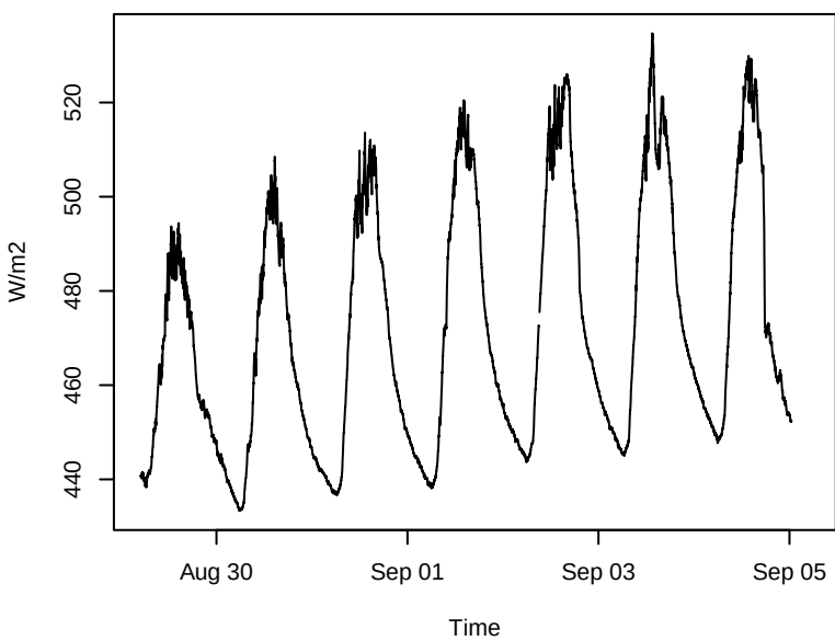
Longwave Down
