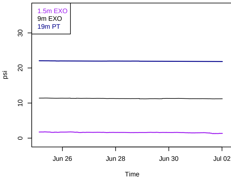
Sonde Pressure
