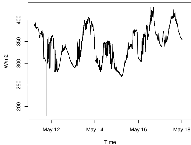
Longwave Up
