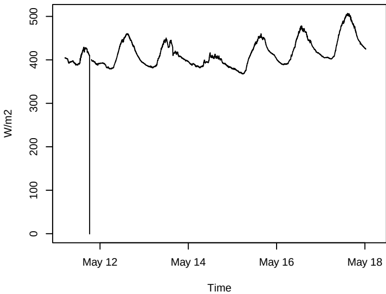
Longwave Down
