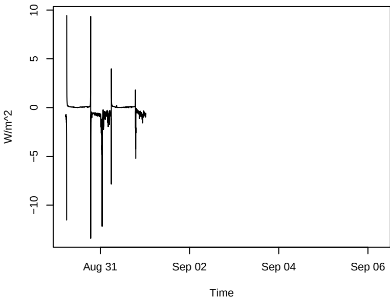
Albedo
