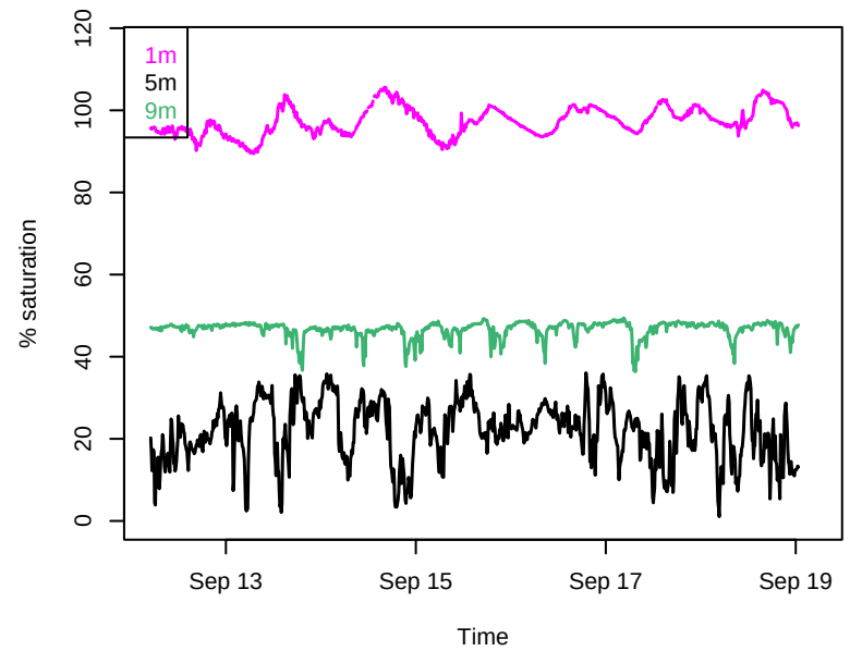
DO % saturation
