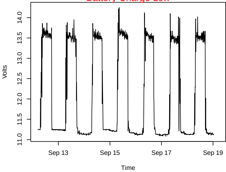
Campbell Logger Battery Battery Charge Low
