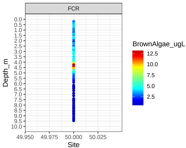
BrownAlgae_ugL 2026-09-15
