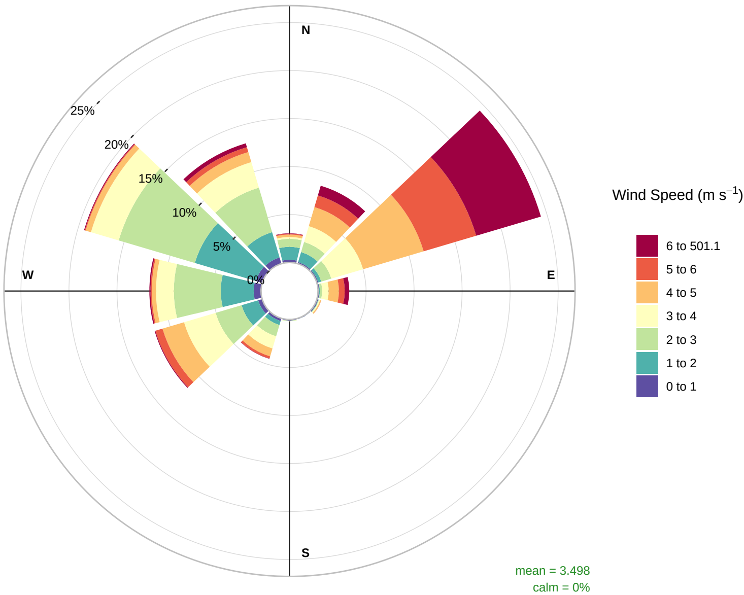
Wind Rose – Last 7 Days
