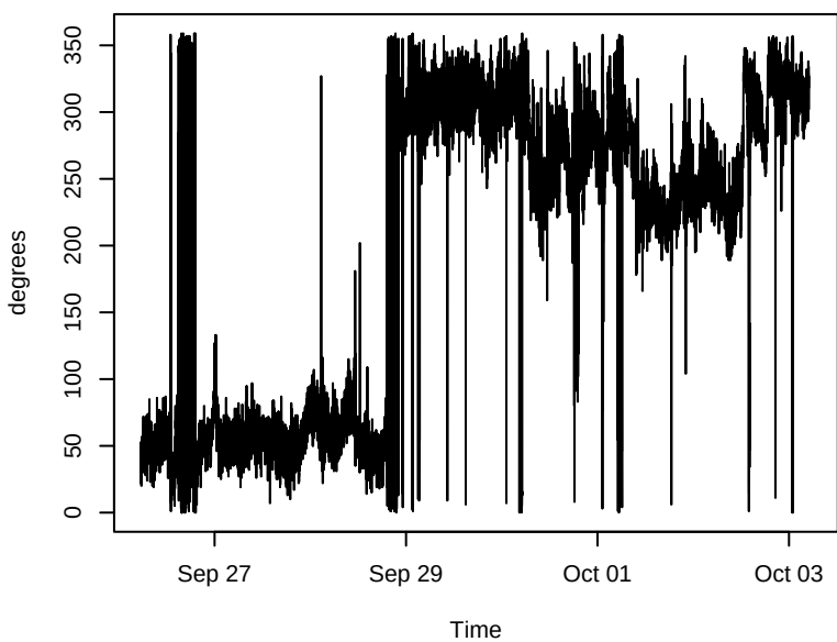
Corrected Wind Direction
