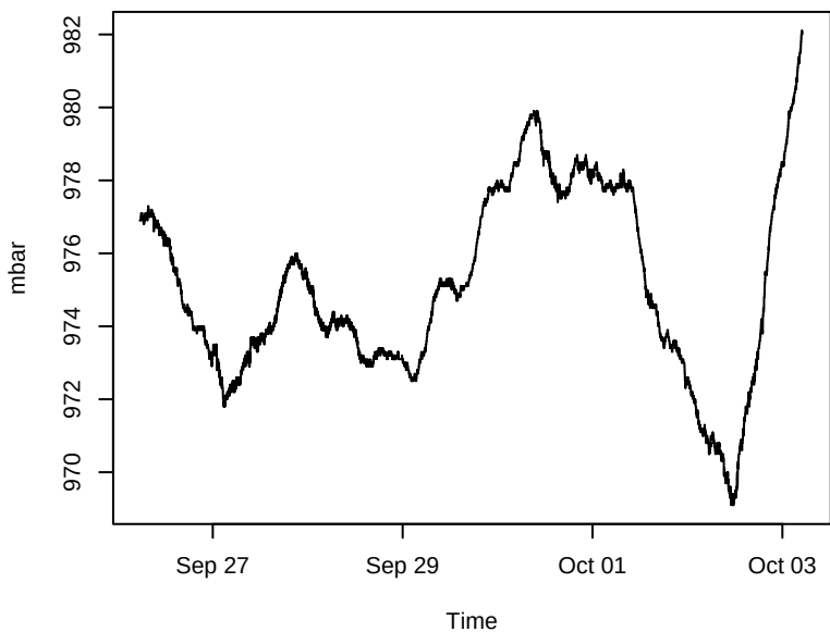
Barometric Pressure
