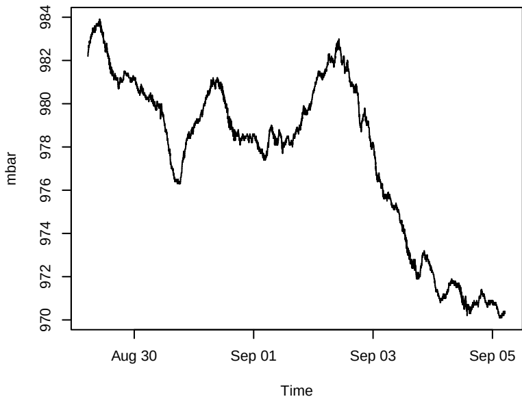
Barometric Pressure
