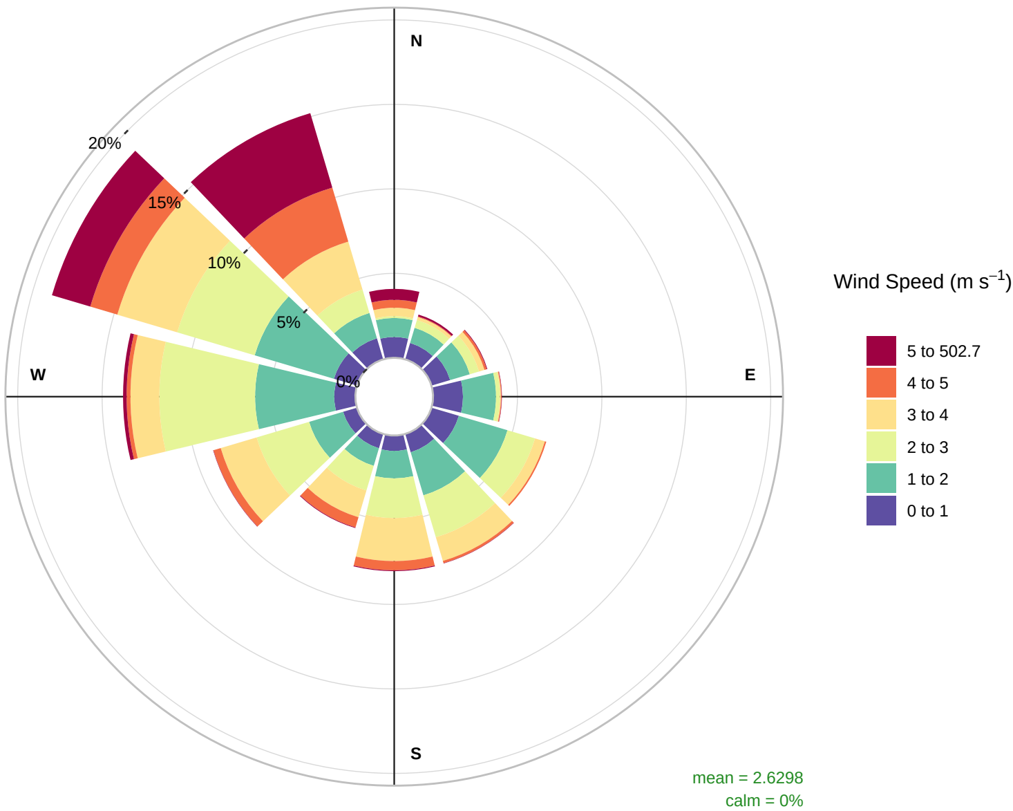
Frequency of counts by wind direction (%)
