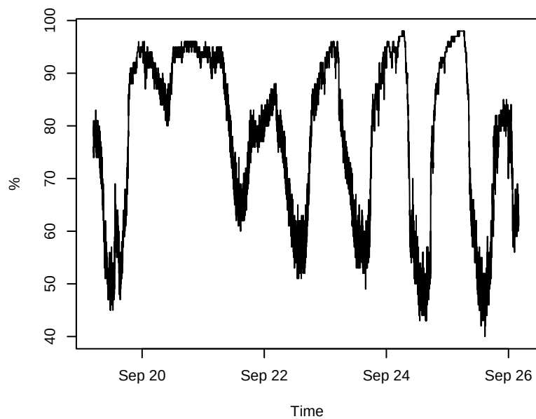
Rel Hum
