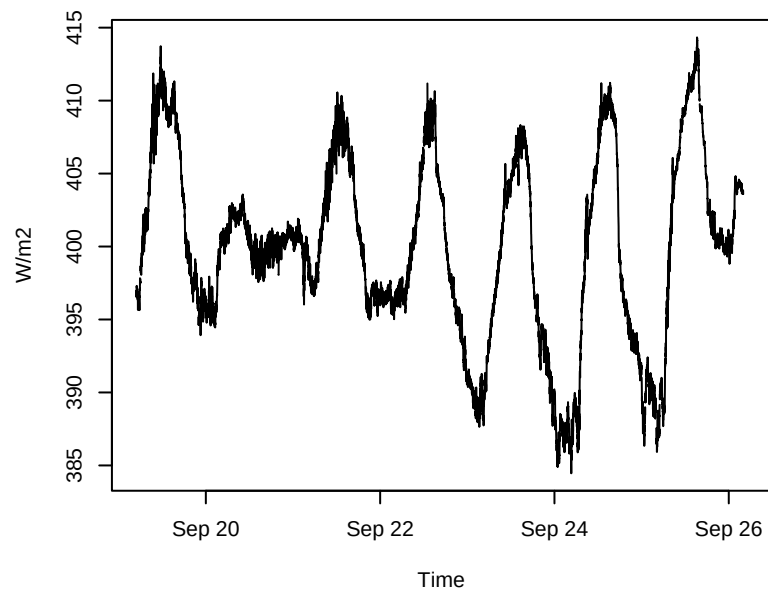
Longwave Down
