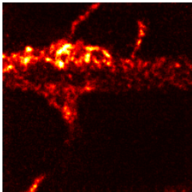
Pix2Pix
