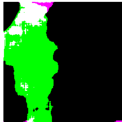
Rings: 0.65, Fibres: -1.00
