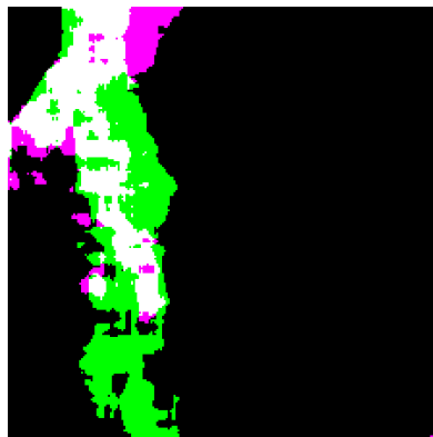
Rings: 0.62, Fibres: -1.00
