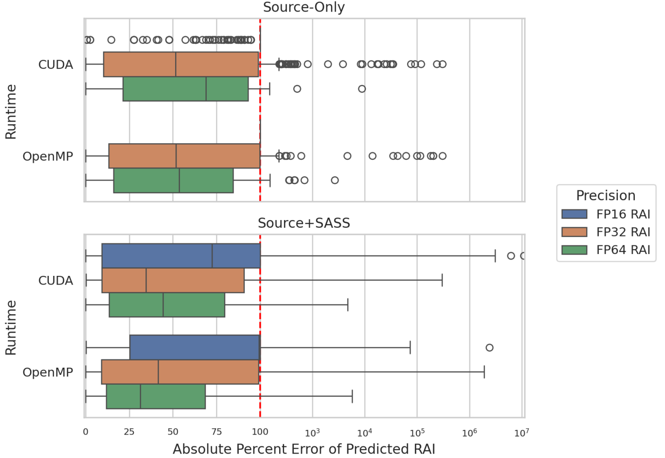
Fig. 7. Absolute percent error on nonzero RAI cases, stratified by runtime. The runtime split is precision-sensitive rather than uniform: CUDA tends to be easier for FP16/FP32 triage, while FP64 remains mixed across CUDA and OpenMP.
