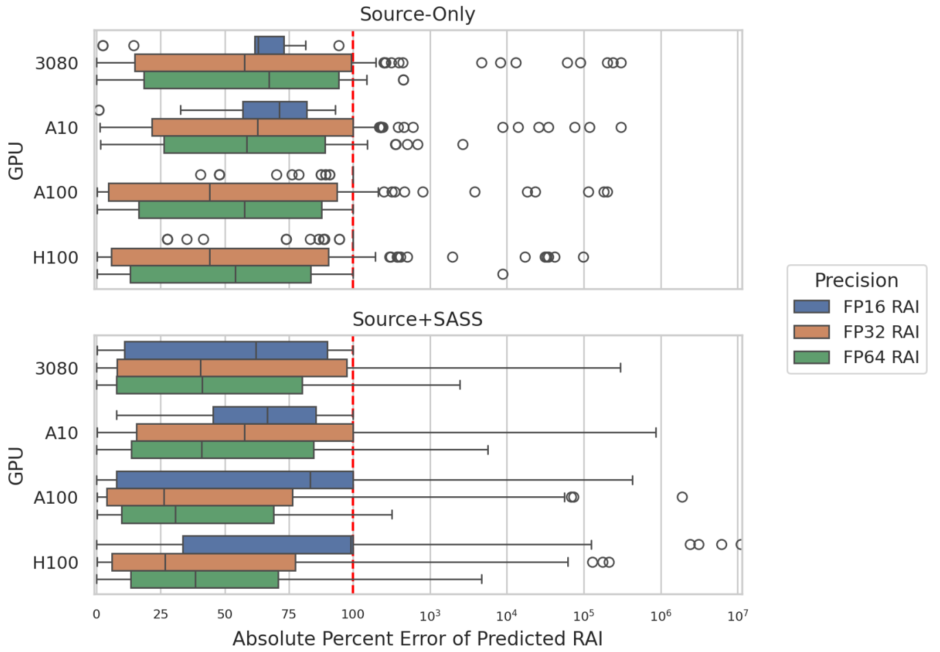
Fig. 6. Absolute percent error on nonzero RAI cases, stratified by GPU. The smaller-cache 3080/A10 settings are generally less stable than A100/H100, especially for source-level reasoning about FP32/FP64 DRAM-visible traffic.
