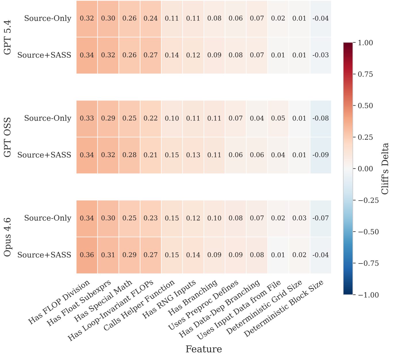
Fig. 8. Exploratory feature/error association heatmap from the released artifact. Positive Cliff’s delta means higher absolute RAI error when the feature is present. The strongest repeated error signals come from division, special math, reusable subexpressions, and loop-invariant floating-point work. A post-hoc Mann–Whitney/BH sanity check across the same 72 model×prompt×feature cells preserves repeated positive associations for division, common float subexpressions, special math, loop-invariant FLOPs, helper-function calls, RNG inputs, branching, preprocessor defines, and data-dependent branching; those features appear in 7–90% of the 1,336 voted kernels. Because the feature labels are generated by an auxiliary LLM-voting pipeline, we treat this figure as descriptive rather than causal.
