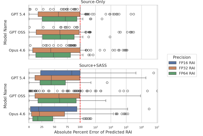
Fig. 5. Absolute percent error on nonzero RAI cases, by model, precision, and evidence setting. The distribution has both a useful low-error region and a long failure tail. source+SASS sharply expands the low-error FP16 region for the frontier models and tightens many FP32/FP64 distributions, mirroring the classification gains.
