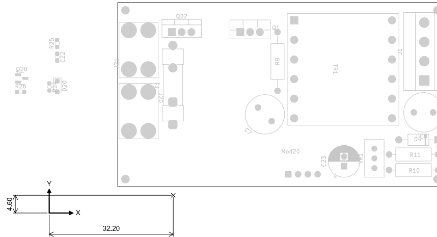
Top Test Points (Scale 1:1)
