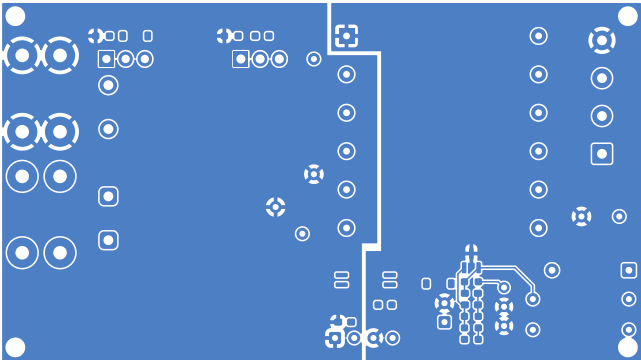
L2 (Sig, PWR) (Scale 1:1)
