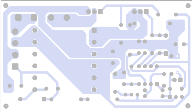
Bottom Assembly (Scale 1:1)
