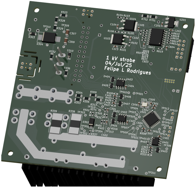
Bottom View
