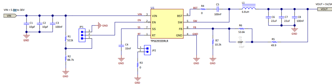
Figure 10-1. TPS62933 5-V Output, 3-A Reference Design
