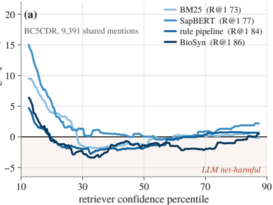
local net \Delta Accuracy@1 of the LLM stage (points)
