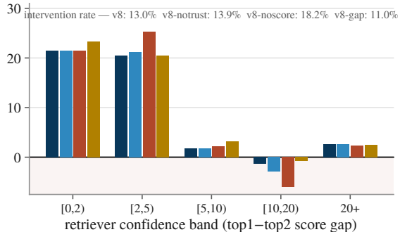
BioRED
