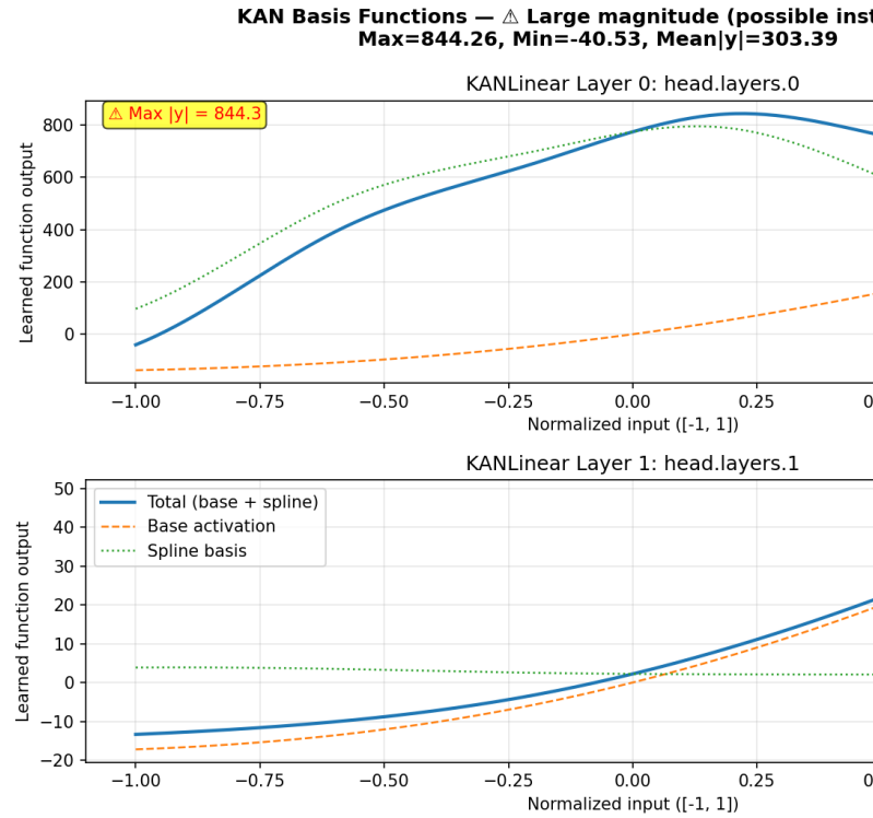
Fig. 1. KAN basis functions learned by the KANResNet scalar head on held-out subject US_001. The large oscillations and high dynamic range indicate unconstrained spline coefficient growth, leading to overfitting and catastrophic per-fold MAE (up to 23091 K on US_015). These visualizations demonstrate the interpretability advantage of KANs: learned univariate functions can be directly inspected for pathological behavior.
