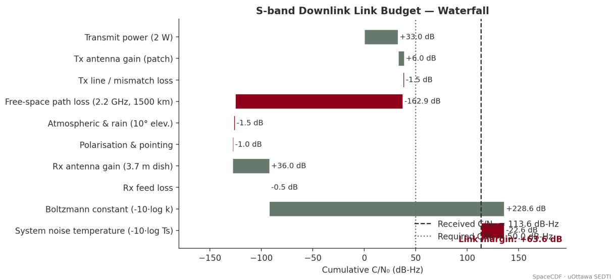
Figure — S-band downlink link-budget waterfall.
