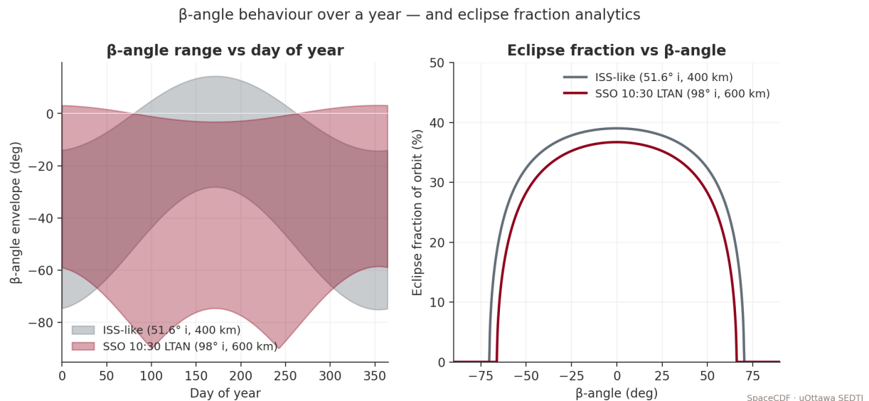
Figure — Eclipse fraction analytics for thermal envelope.
