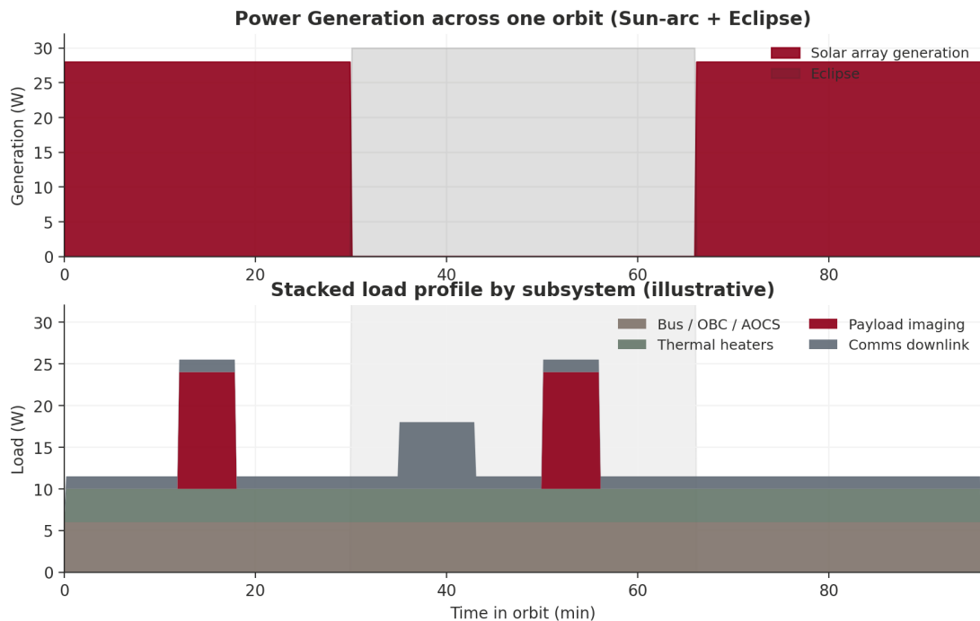
Figure — Power generation and stacked load profile.
