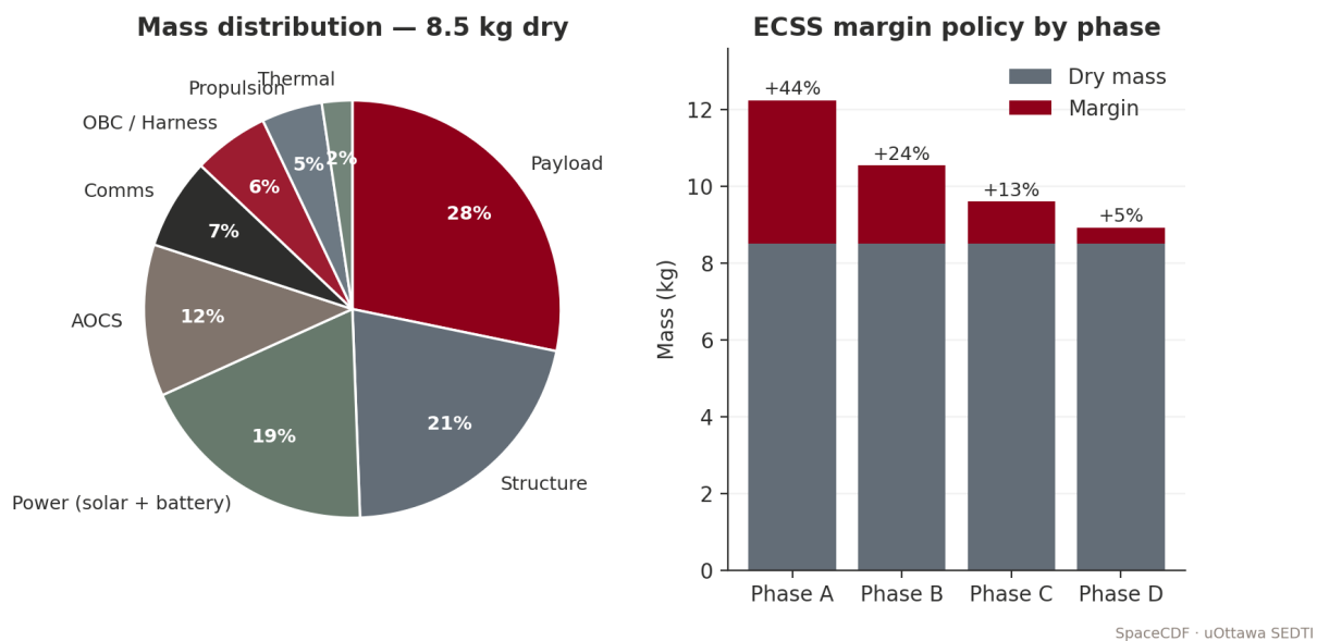
Figure — Mass distribution and ECSS margin policy.
