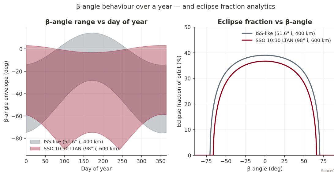
Figure — \beta -angle envelope and eclipse fraction.
