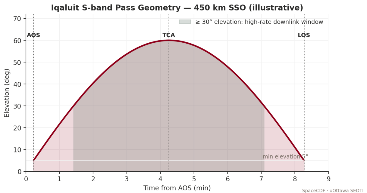
Figure — Iqaluit S-band pass geometry.
