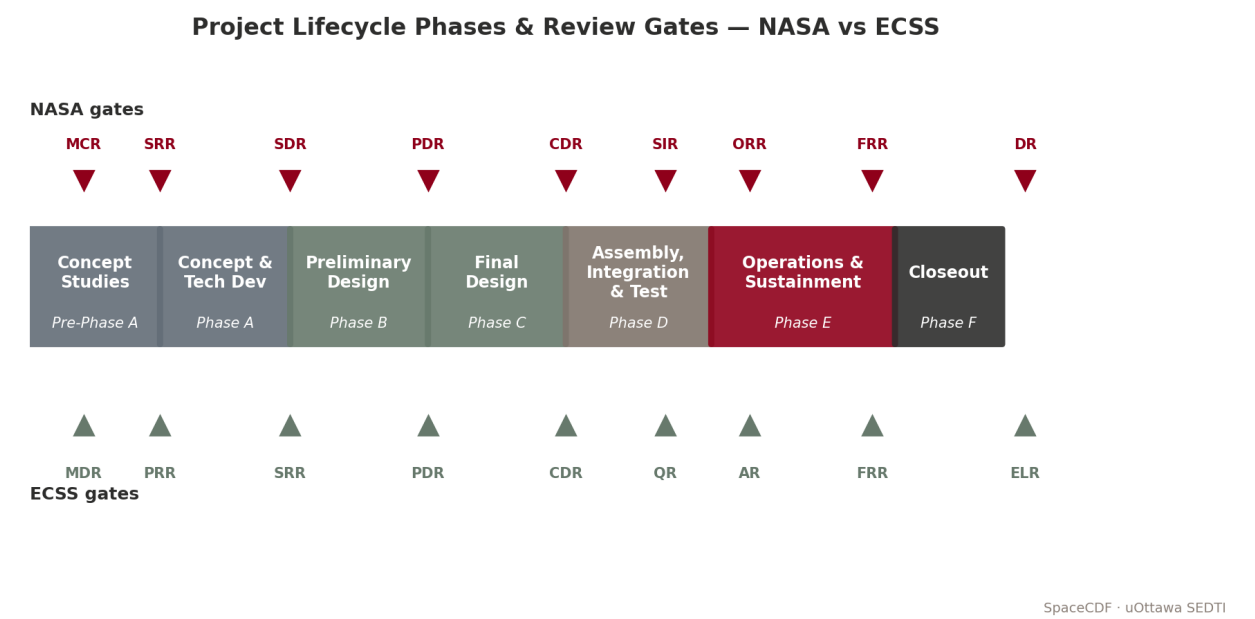
Figure — Lifecycle phases and review gates.
