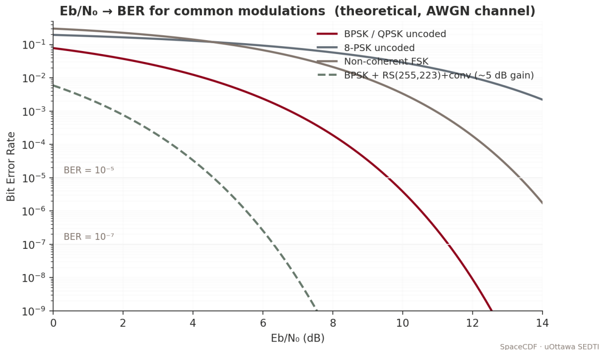
Figure — E_b/N_0 vs BER for common modulations.
