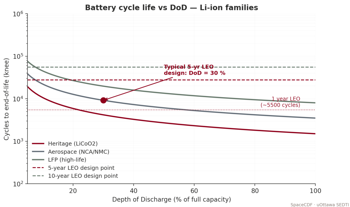
Figure — Battery cycle life vs DoD.
