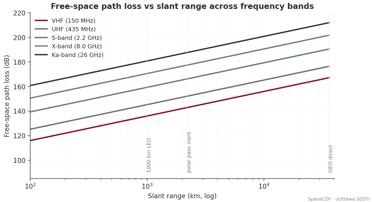
Figure — Free-space path loss vs slant range across bands.
