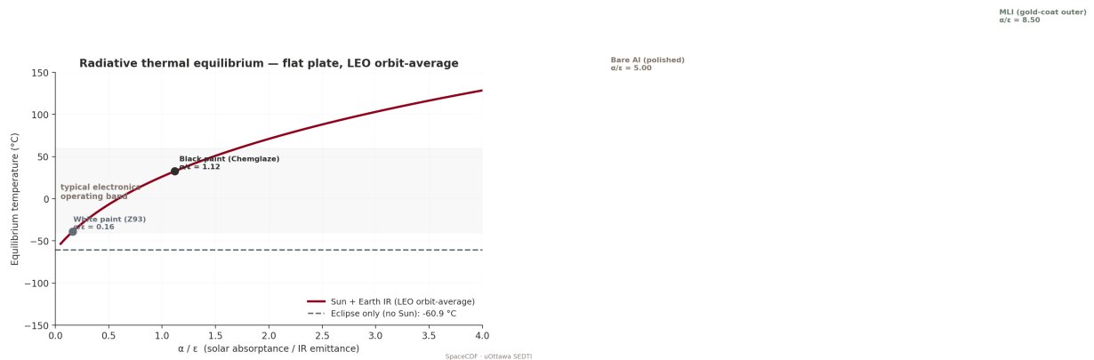
Figure — Radiative thermal equilibrium vs \alpha/\epsilon .
