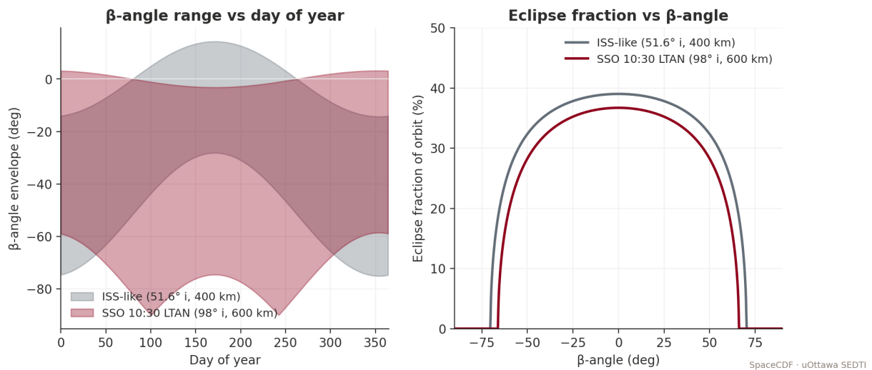
FIGURE 24 — \beta -angle envelope and eclipse fraction analytics.
