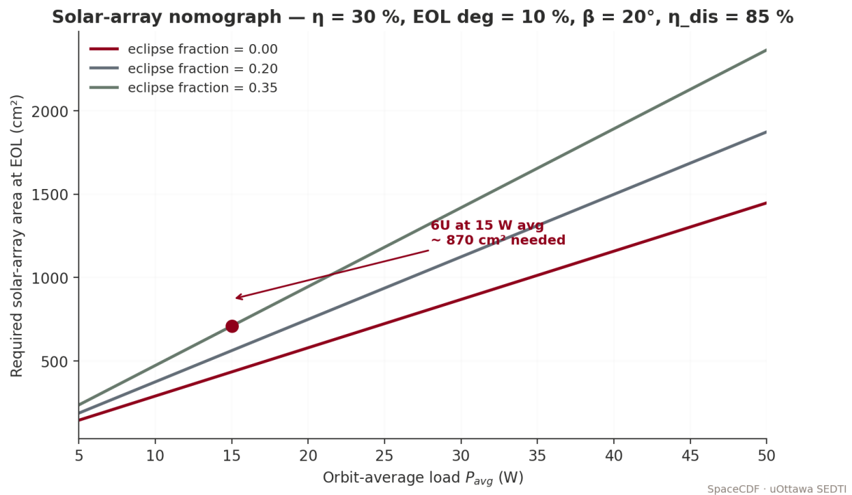
FIGURE 20 — Solar-array sizing nomograph.
