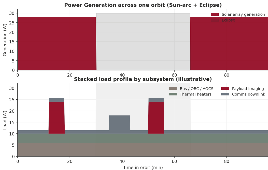
FIGURE 19 — Power generation and stacked load profile.
