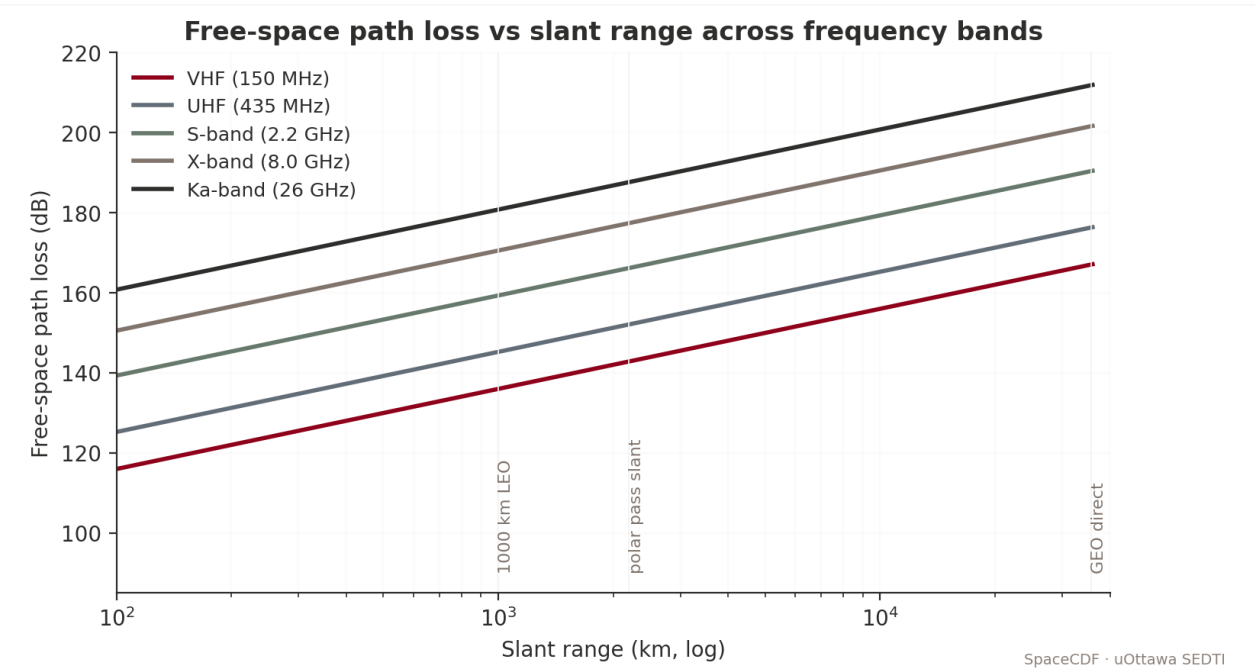
FIGURE 29 — Free-space path loss vs slant range across bands.
