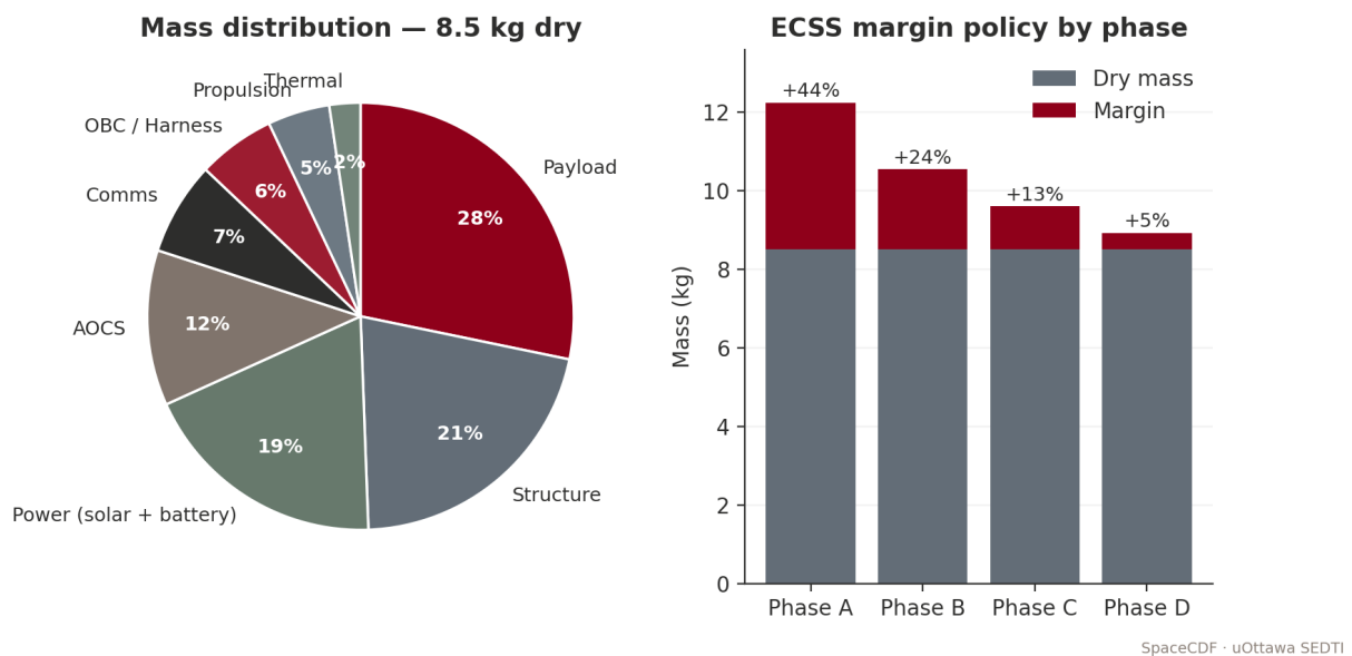
FIGURE 23 — Mass distribution and ECSS margin policy.
