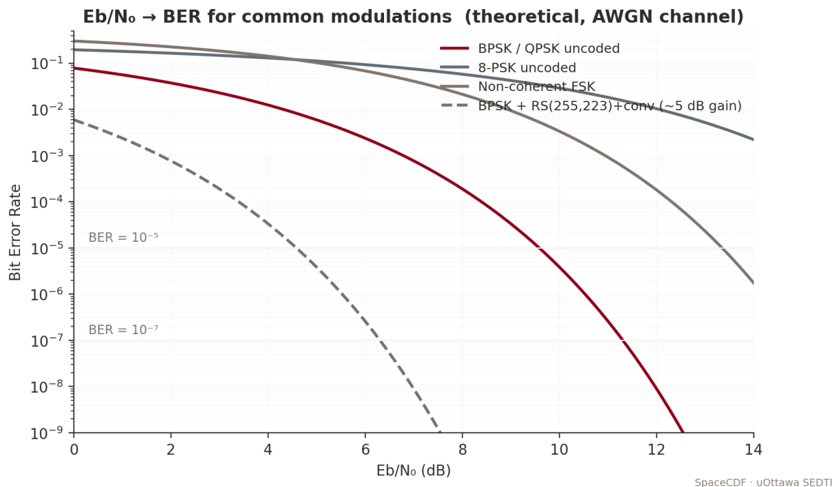
FIGURE 31 — E_b/N_0 vs BER for common modulations.
