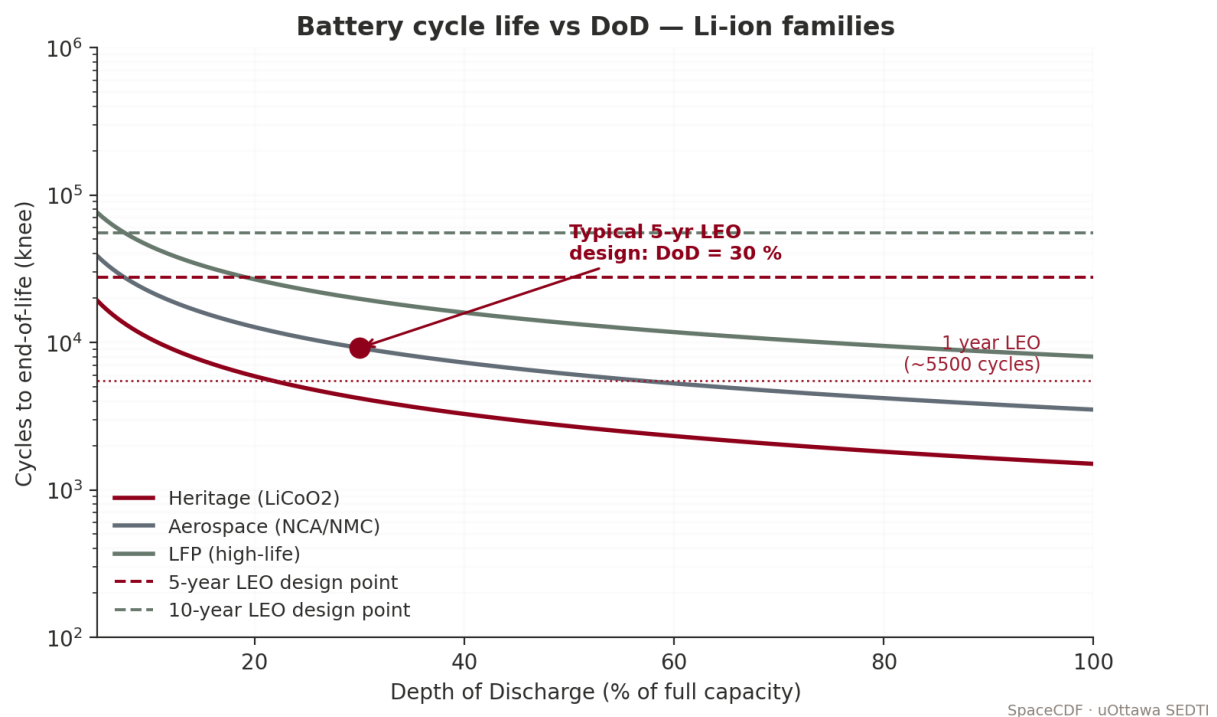
FIGURE 21 — Battery cycle life vs DoD.
