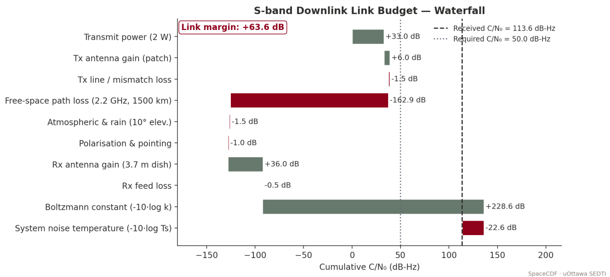
FIGURE 27 — S-band downlink link-budget waterfall.
