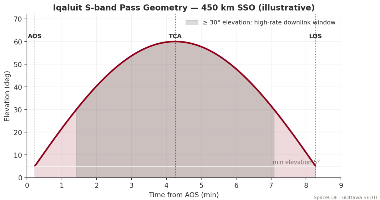
FIGURE 28 — Iqaluit S-band pass geometry.
