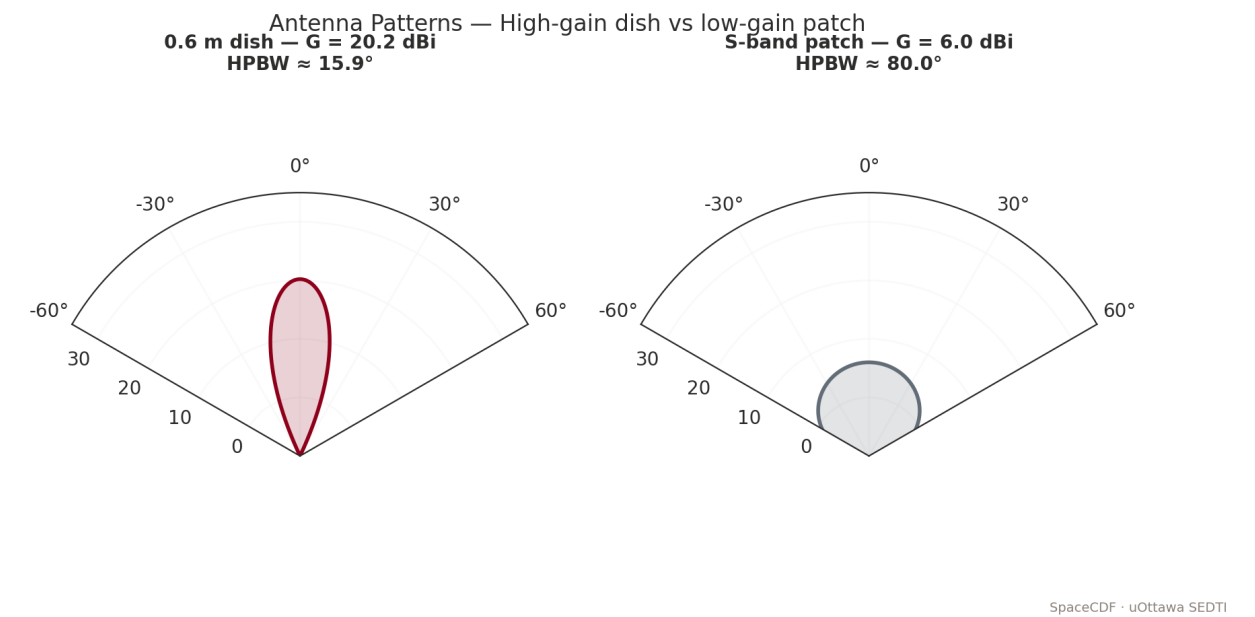
FIGURE 30 — Antenna patterns: high-gain dish vs patch.
