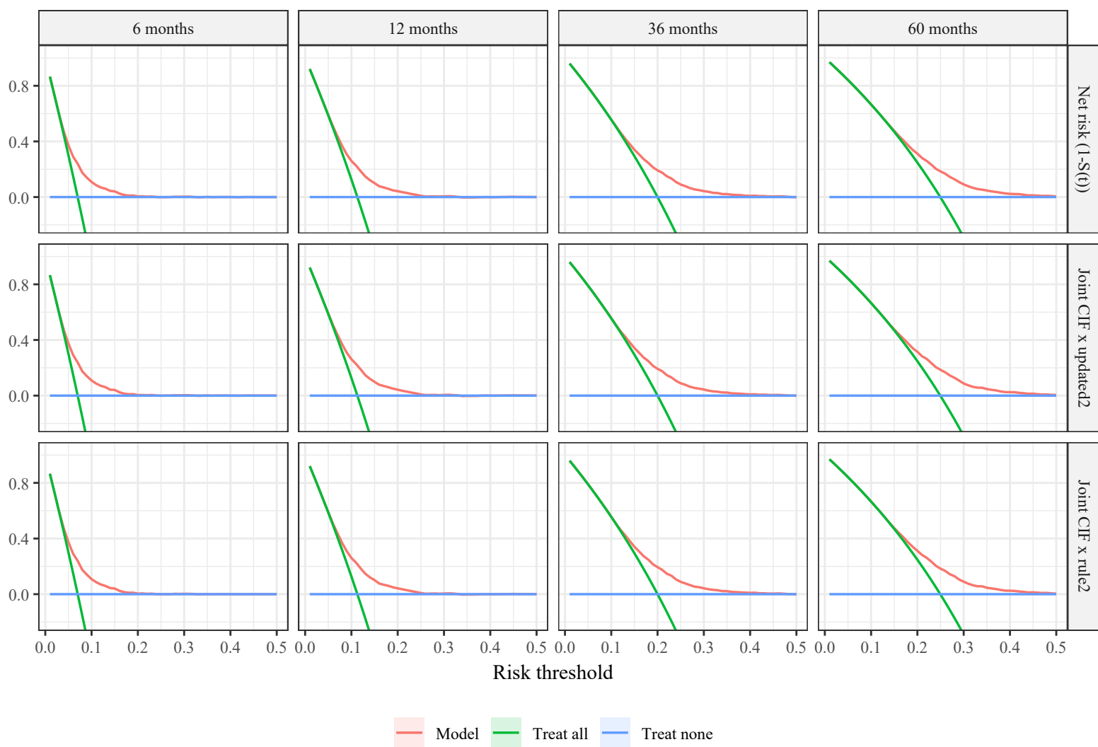
Standardized net benefit
