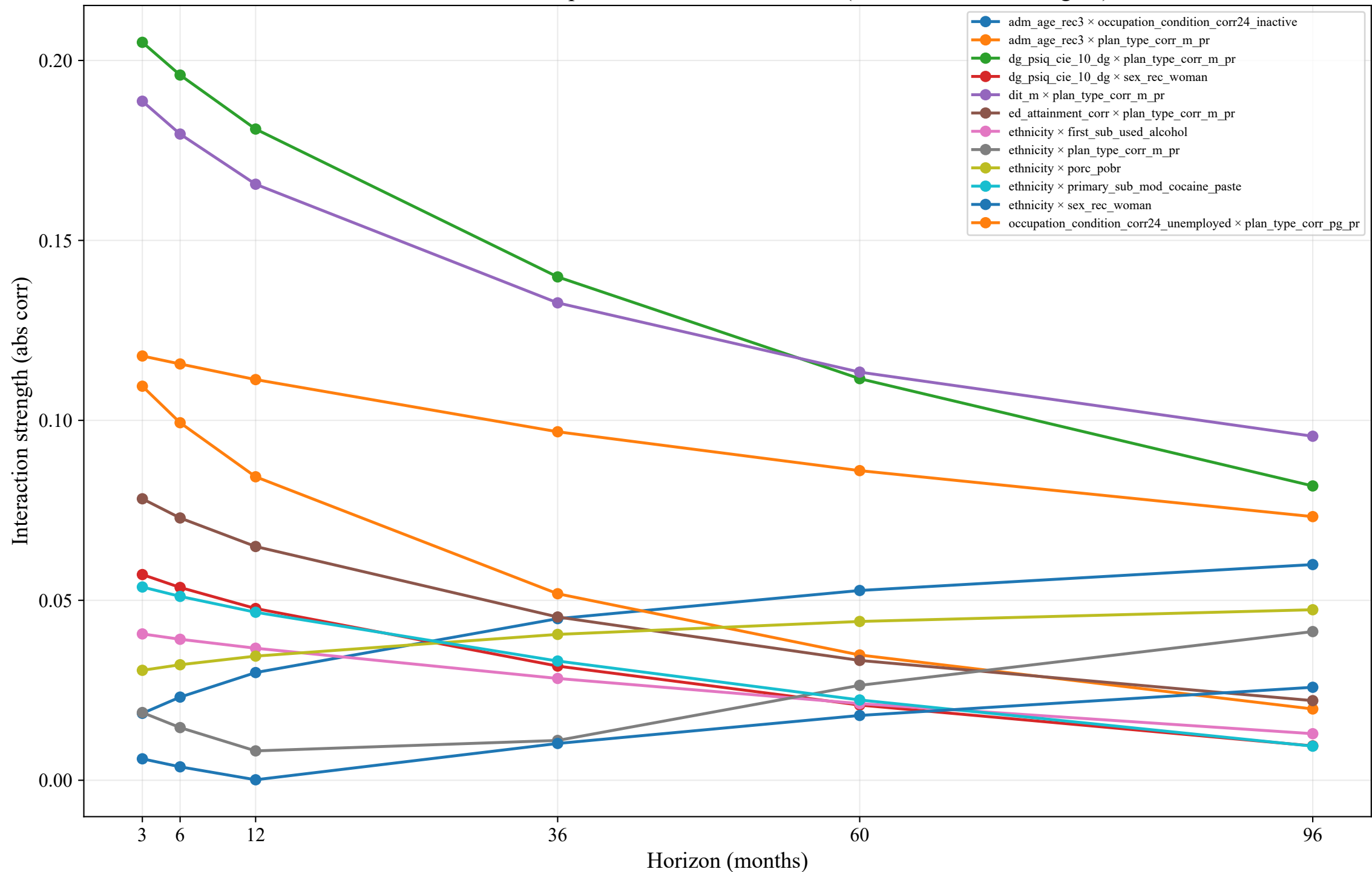
Readmission: Time-Dependent Interaction Profiles (abs corr of residual signal)
