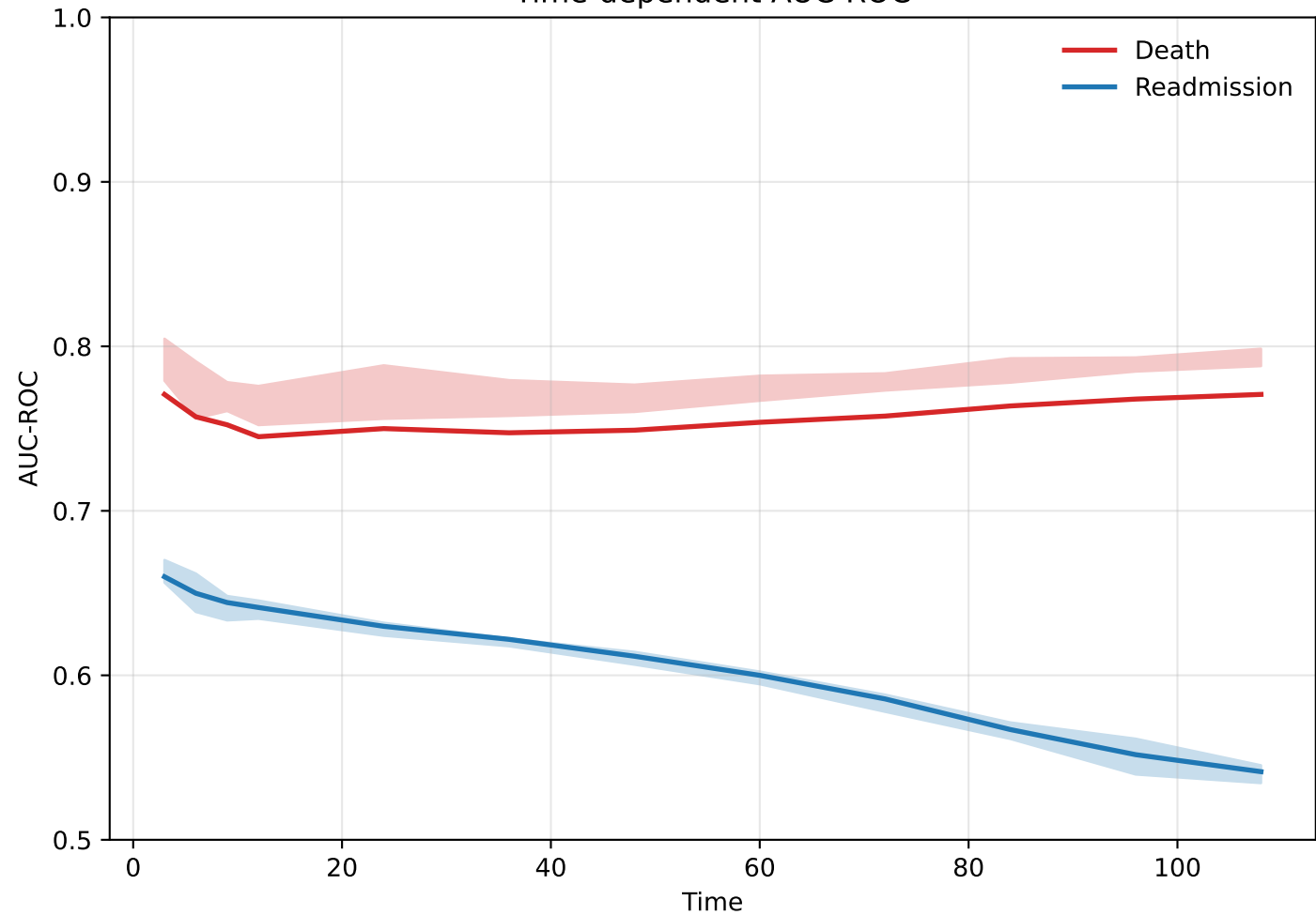
Time-dependent AUC-ROC
