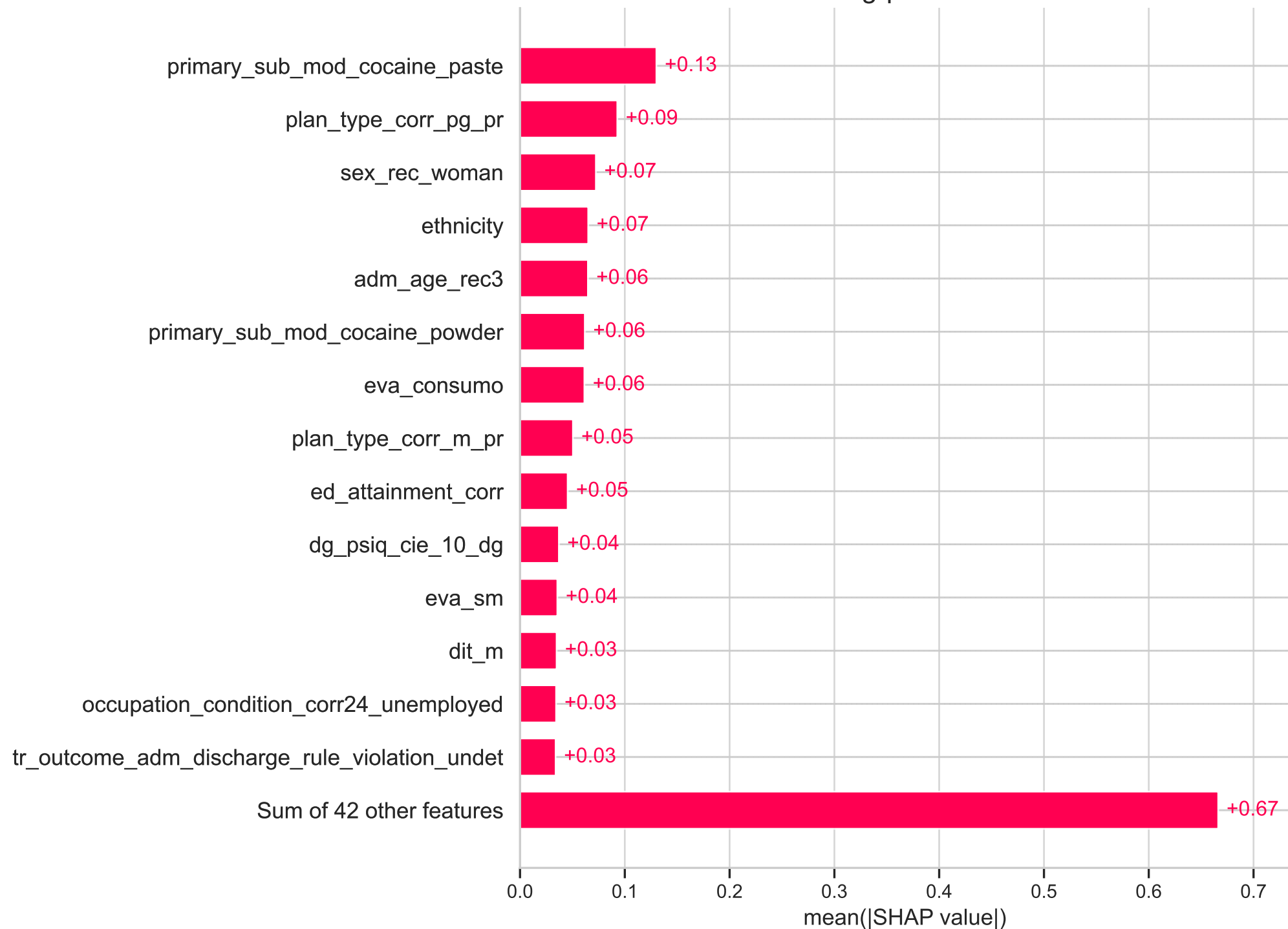
Feature Importance (Readmission - 6m) Scale: log-partial hazard
