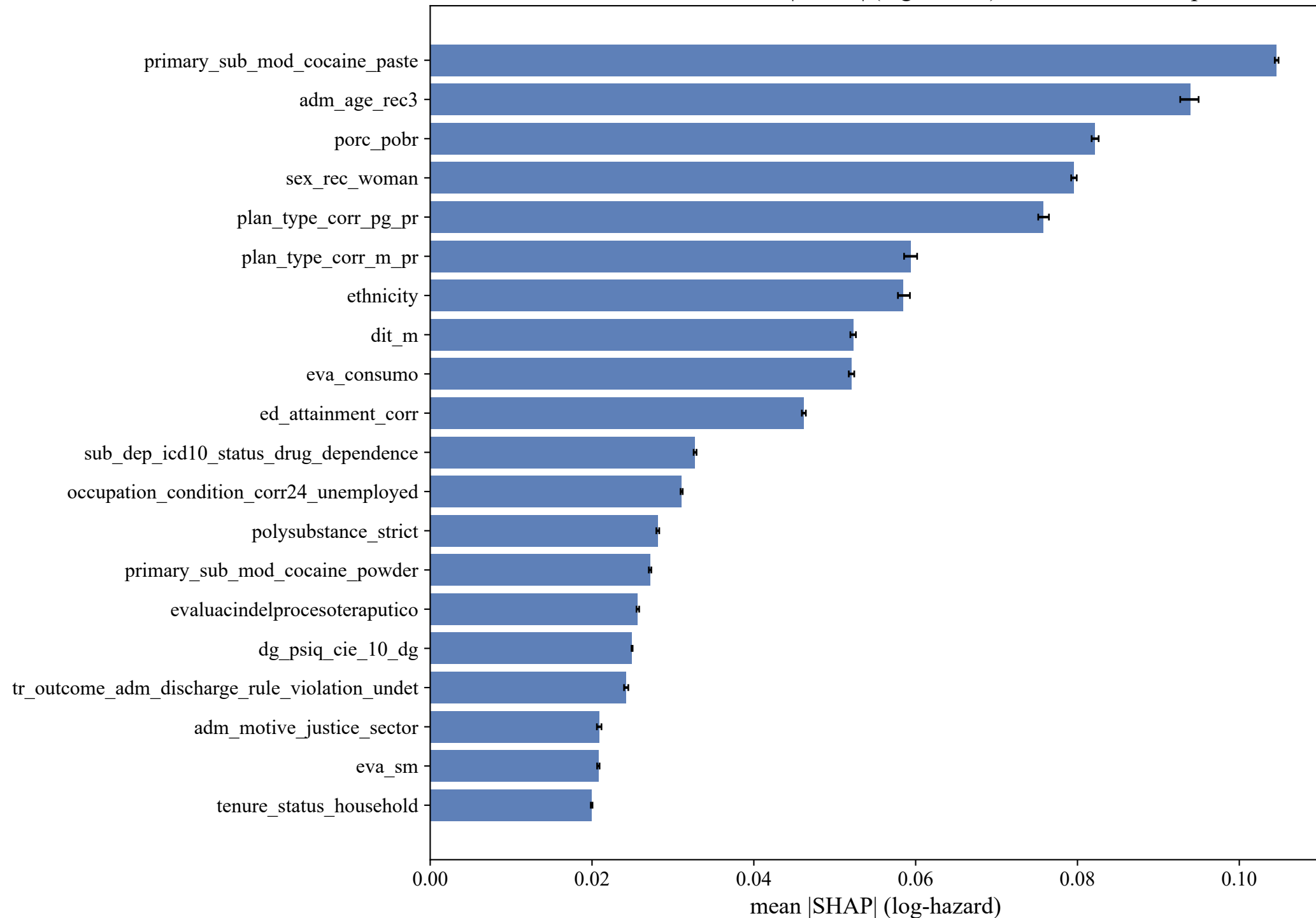
Readmission Global mean |SHAP| (log-hazard) with 95% bootstrap CI
