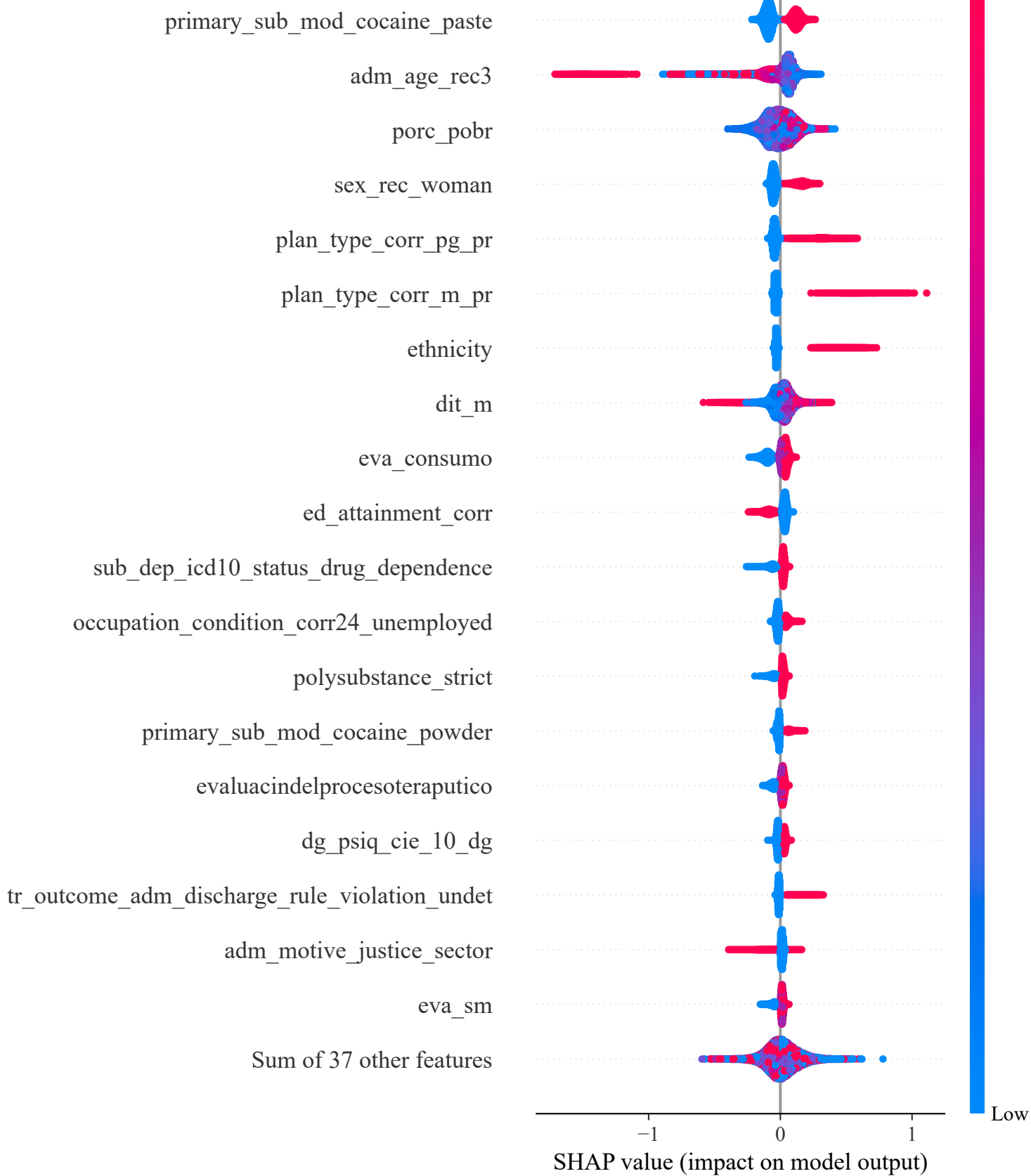
Readmission SHAP Beeswarm (log-hazard scale)
