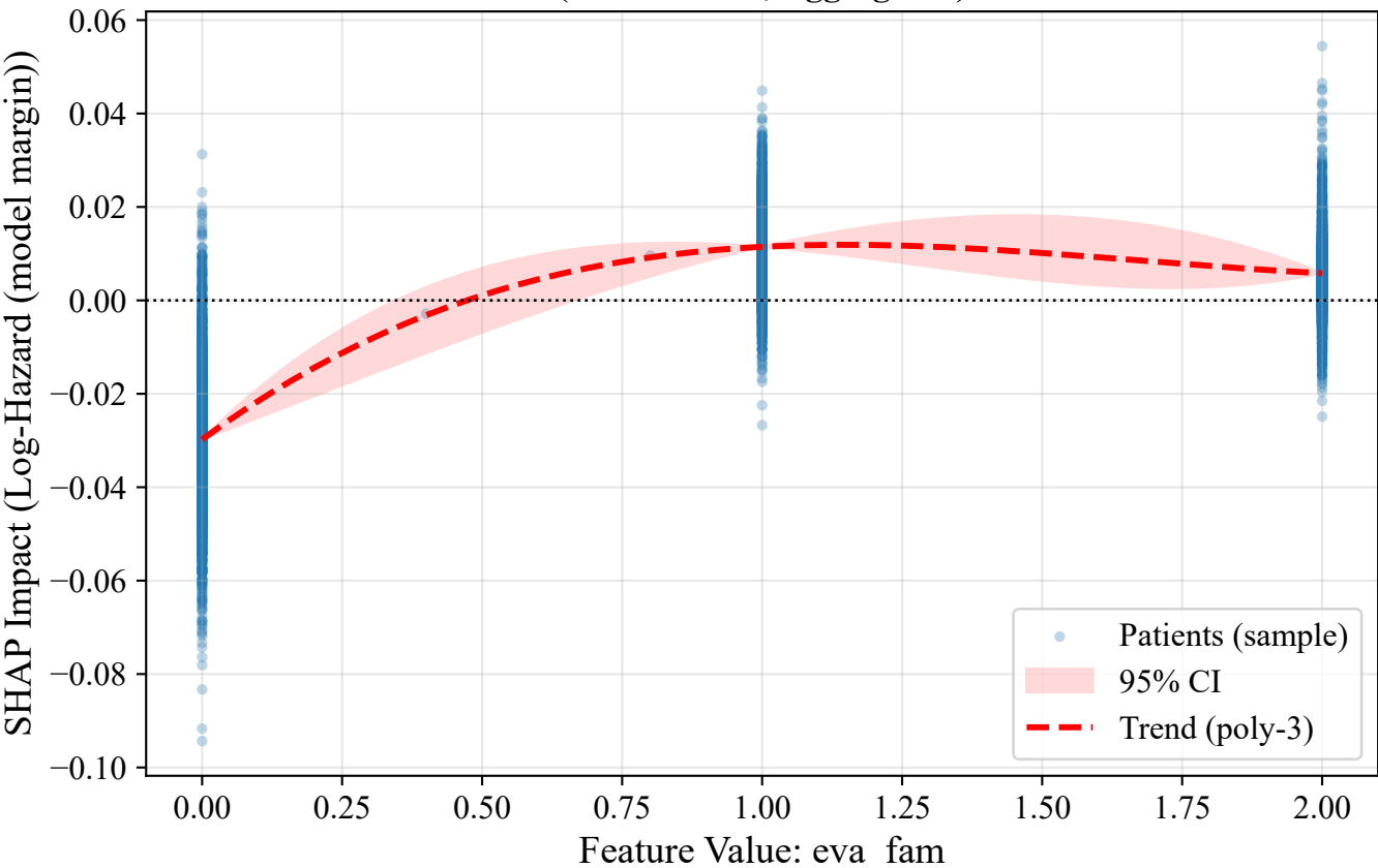
Functional Form: eva_fam (Readmission, Aggregated)
