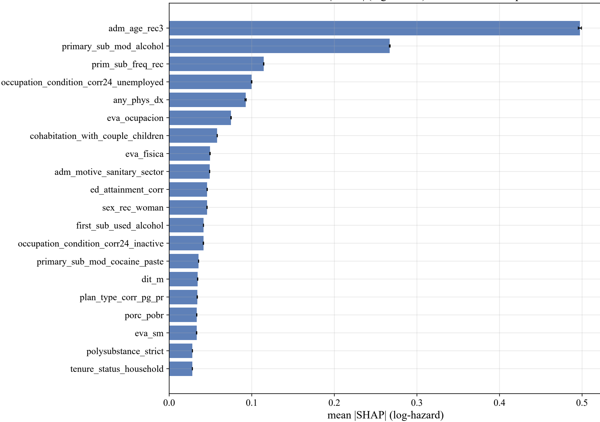
Death Global mean |SHAP| (log-hazard) with 95% bootstrap CI
