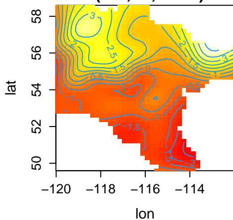
s(lon,lat,35.68)
