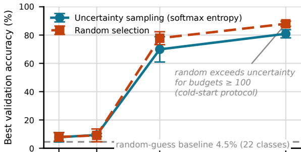
(a) cold-start scorers
