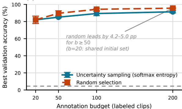
(b) warm-started in-domain scorers
