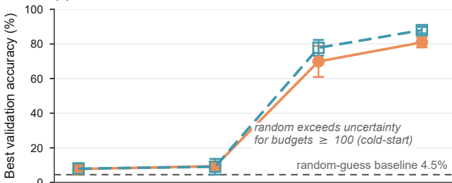
(a) cold-start scorers
