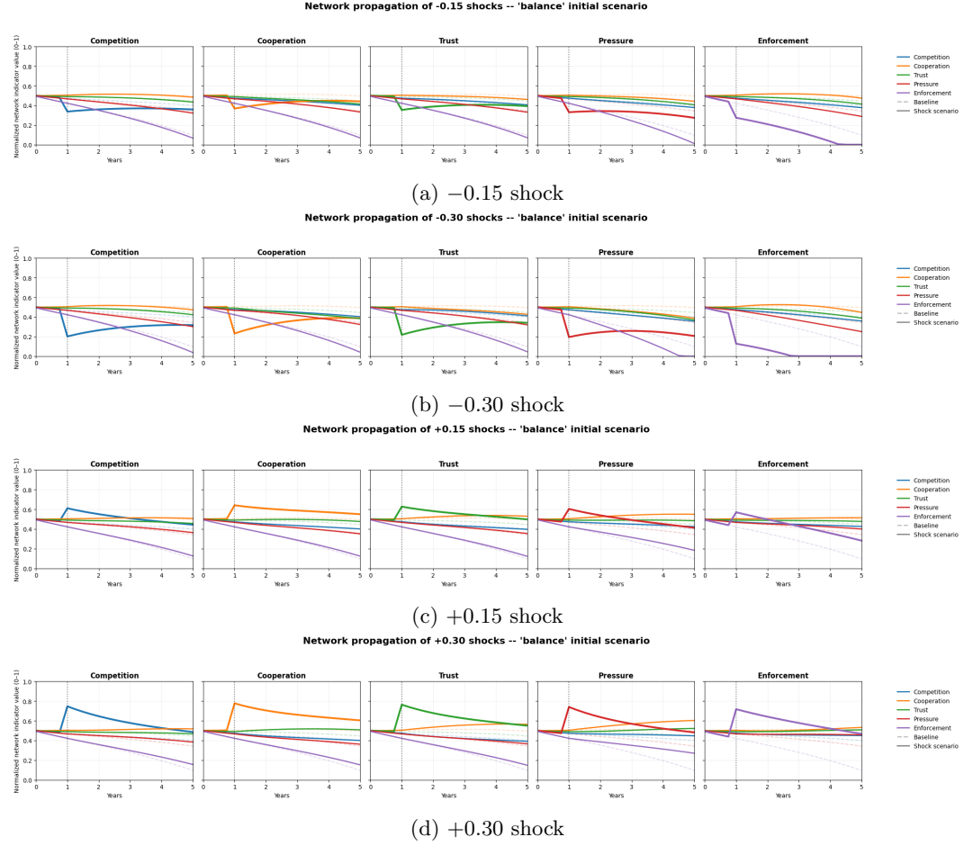
Fig. 12: Time-series response of network indicator values (0–1) over a 5-year period following single-parameter shock interventions for the balance initial scenario. Dashed lines indicate unshocked baseline trajectories; bold solid lines indicate the immediate parameter displacement at Year 1 and subsequent network propagation.
