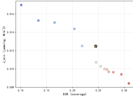
J = 12 (14 sols, r=-0.970 )
