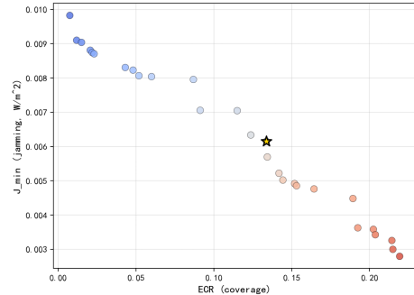
J = 8 (28 sols, r=-0.988 )
