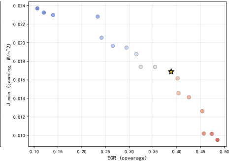
J = 16 (18 sols, r=-0.954 )
