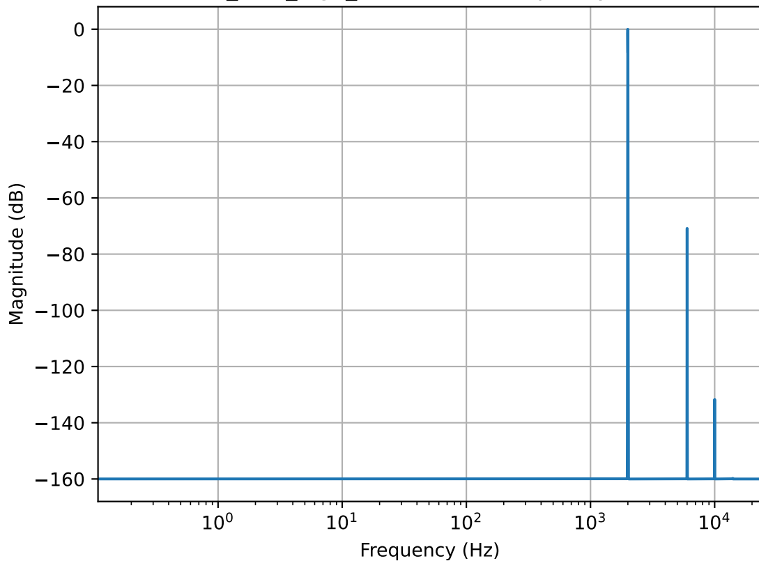
Daniel_5cm_high_harmonics - Frequency Domain
