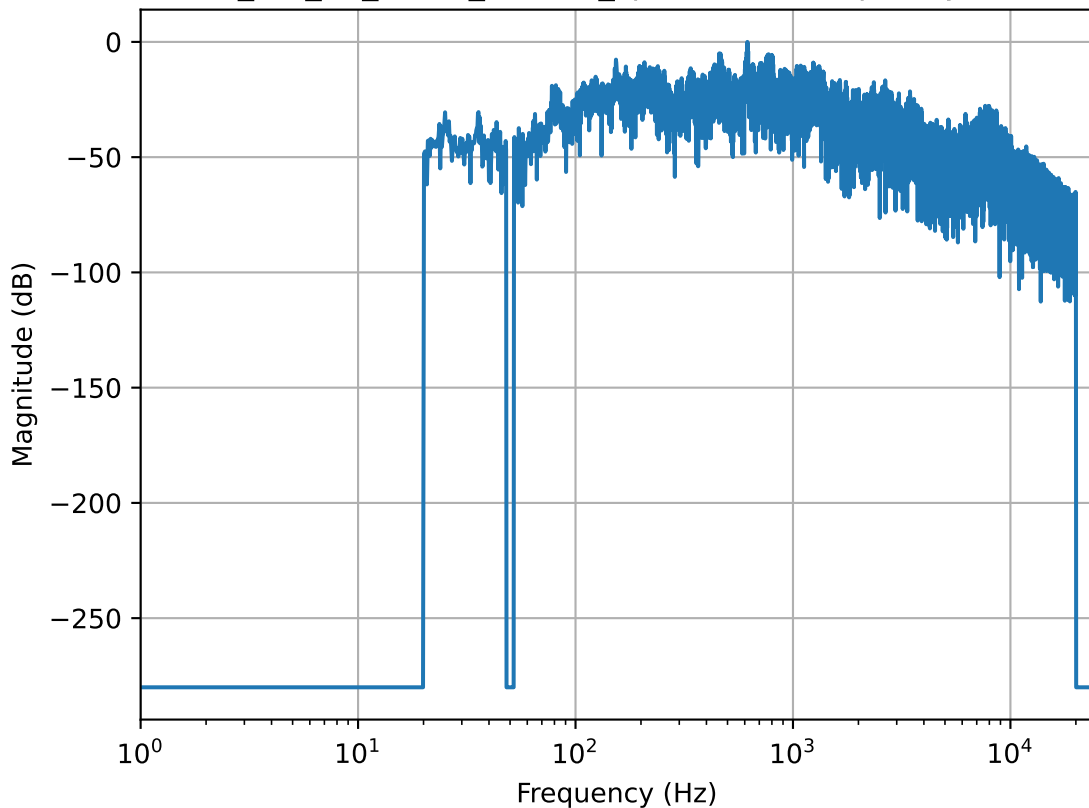
Daniel_1m_03_linear_filtered_spectrum - Frequency Domain
