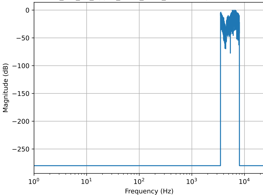
Daniel_1m_06_upper_band_after_tanh - Frequency Domain
