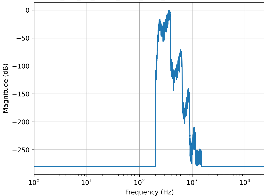
Daniel_1m_07_lower_band_after_tanh - Frequency Domain
