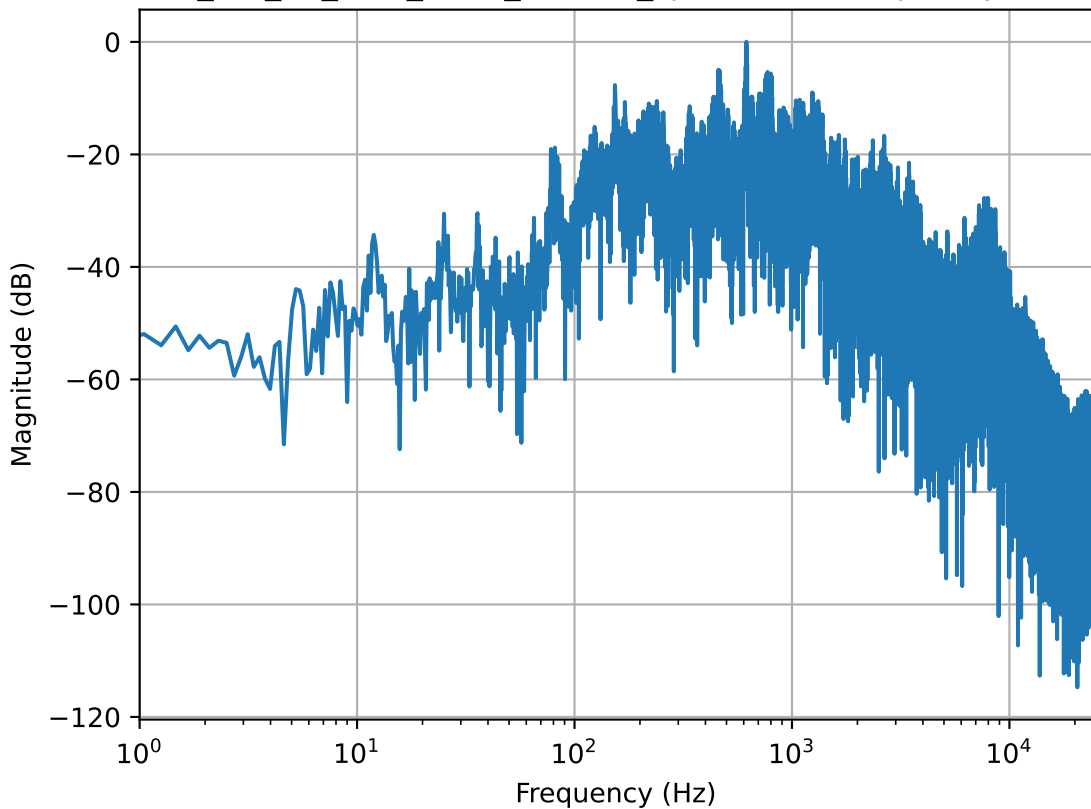
Daniel_1m_08_final_aural_excited_spectrum - Frequency Domain
