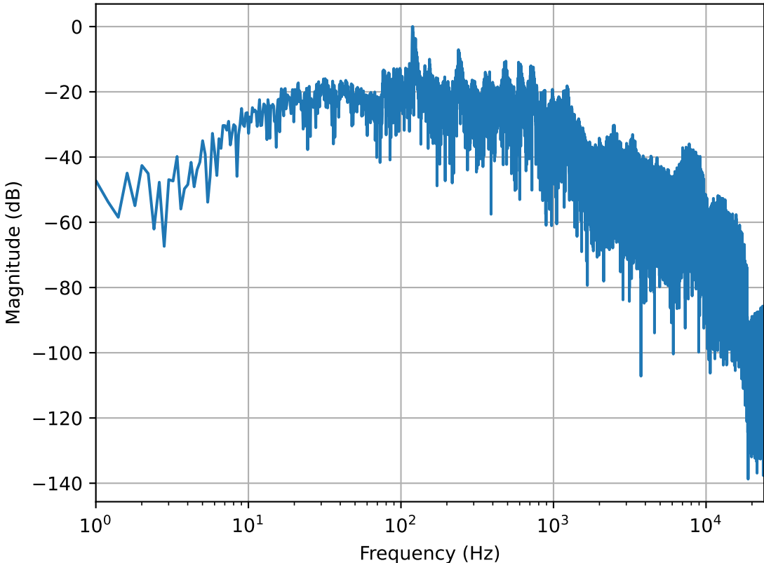
Daniel_5cm_01_original_spectrum_hamming_windowed - Frequency Domain
